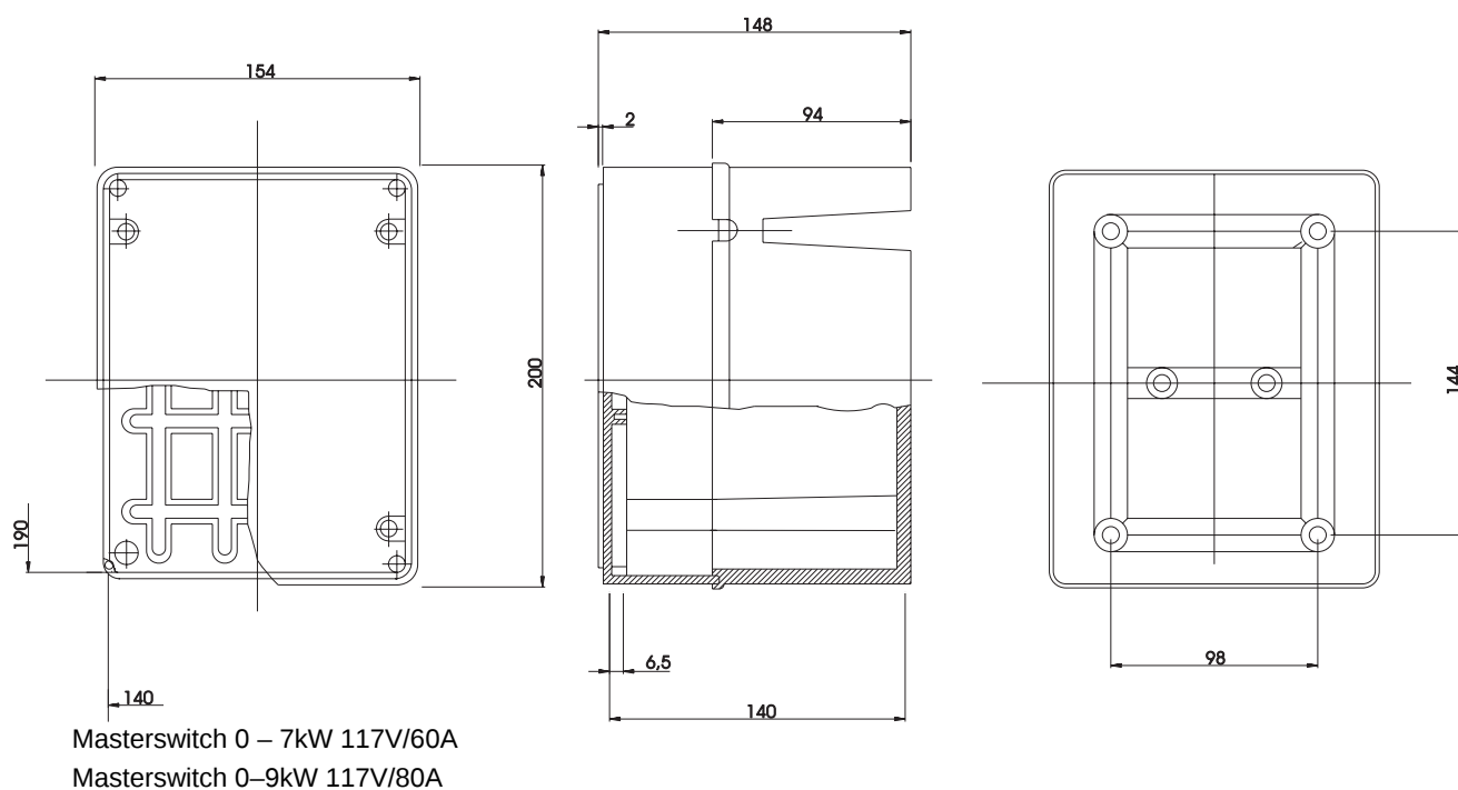
Figure 5: dimensions du Masterswitch 0
